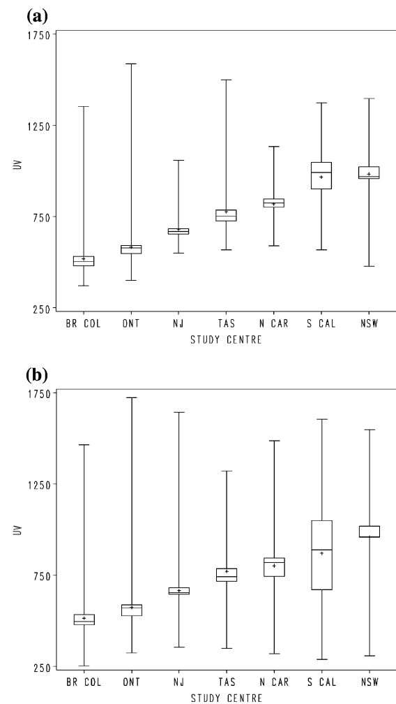
Fig. 1 (a) Average annual lifetime ambient UV irradiance in \text{kJ}/\text{m}^2 at place of residence by study center. (b) Average annual ambient UV irradiance in \text{kJ}/\text{m}^2 at birth and age 10 averaged, by study center. Legend. Mean (+), median (—), interquartile range ( \square ) and range (|); Br Col: British Columbia, Ont: Ontario, NJ: New Jersey, Tas: Tasmania, N Car: North Carolina, S Cal: Southern California, NSW: New South Wales
